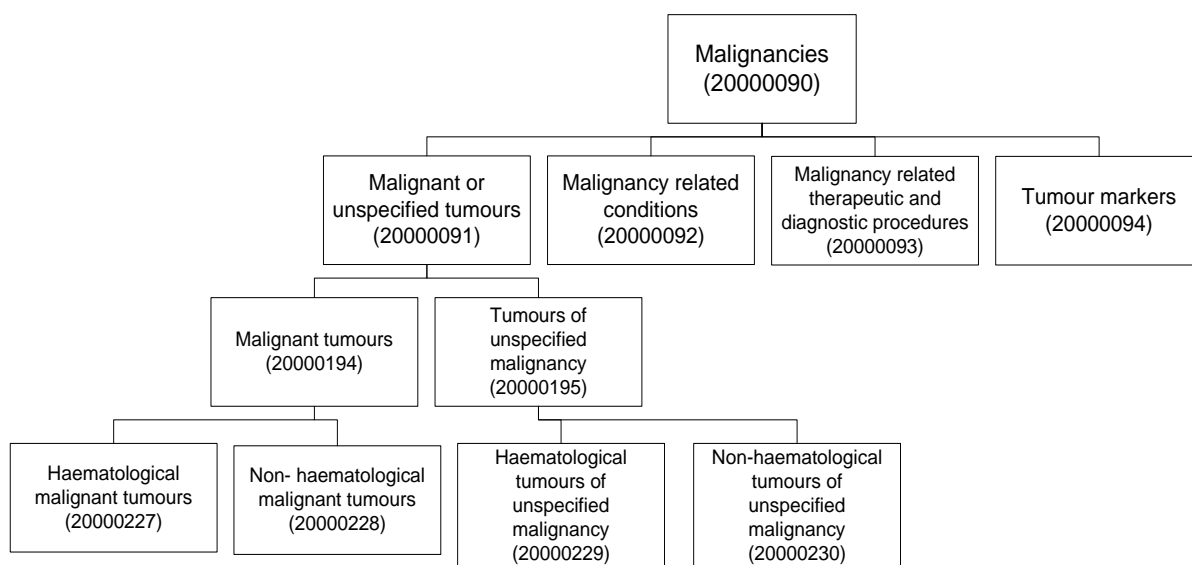
Figure 2-16 Hierarchy Structure of Malignancies (SMQ)
