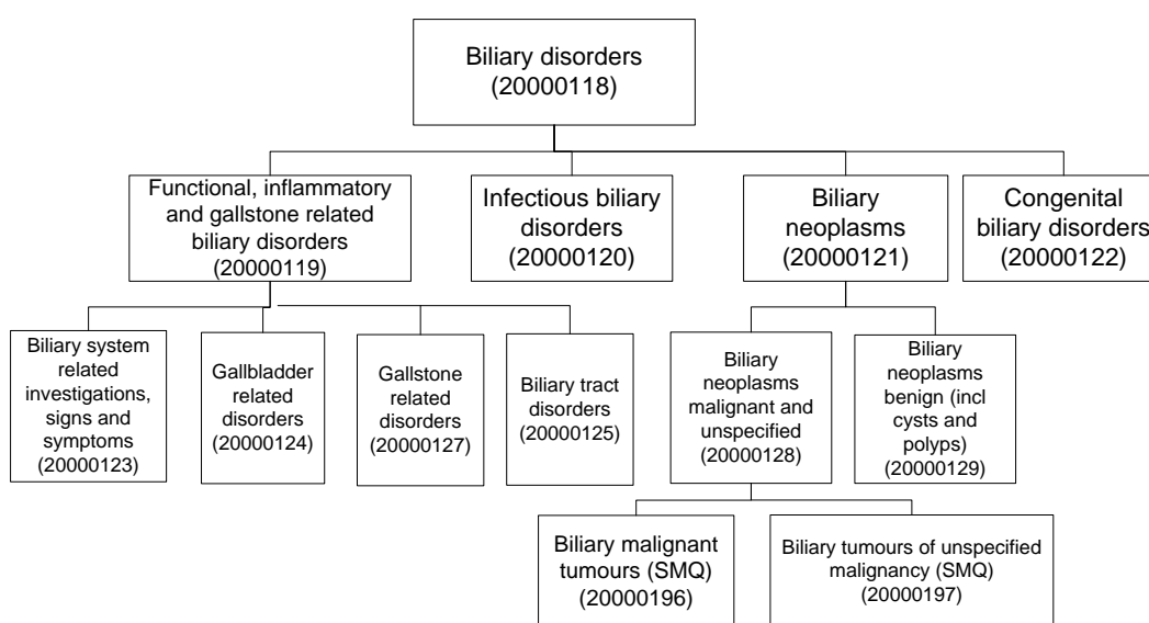
Figure 2-1. Hierarchy Structure of Biliary disorders (SMQ)
