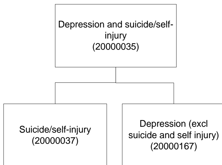
Figure 2-5. Hierarchy Structure of Depression and suicide/self-injury (SMQ)
