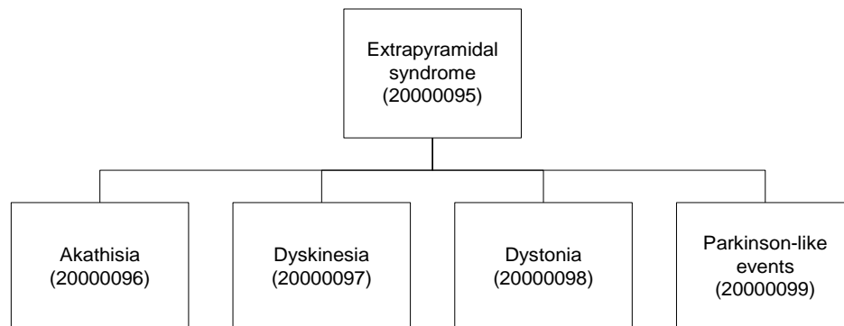
Figure 2-8. Hierarchy Structure of Extraparamidal syndrome (SMQ)
