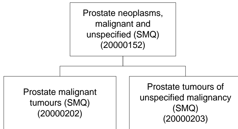
Figure 2-21. Hierarchy Structure of Prostate neoplasms, malignant and unspecified (SMQ)
